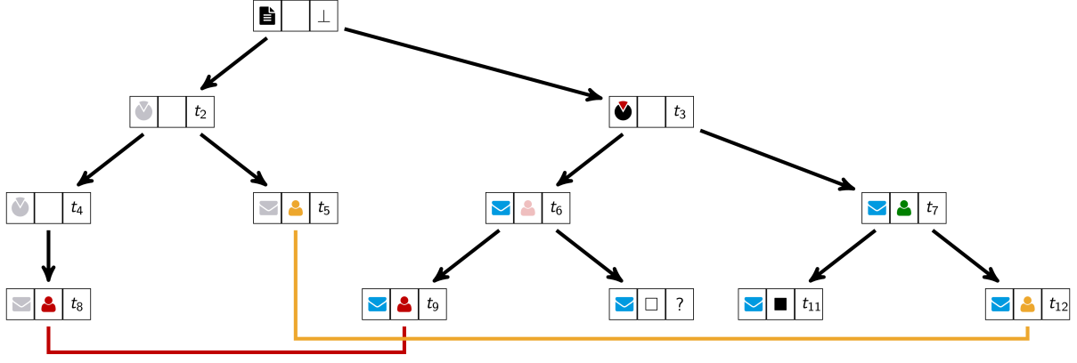
Figure 2. Schematic depiction of a Wikicussion including threads from archived talk pages (indicated by grayed circular segments ☹ dominating archived posts ✉). Each node is represented by a tripartite vector: the first dimension denotes the type of content unit (i.e., a section 📄 or a post ✉), the second the signing author 🧑 (where posts by the same author are denoted by same-color icons such that the corresponding vertices are connected by same-color edges), the third dimension codes the time of creation of the section or post (where ? characterizes unsigned (leaf) nodes of unknown posting time). Unregistered users are denoted by unfilled boxes □, while bots are denoted by filled boxes ■. ⊥ denotes the time of creation of the corresponding Wikicussion.
